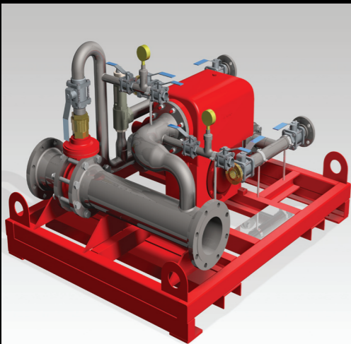
Balance Pressure Proportioning pump skid Foam proportioning and discharge devices
