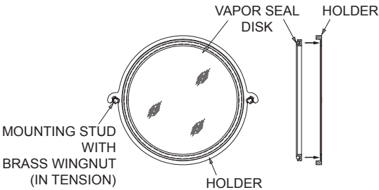
MCS-9 VAPOR SEAL & HOLDER MOUNTING
