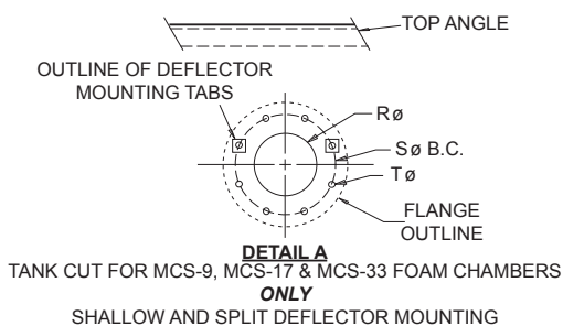
FOAM CHAMBER WITH SPLIT DEFLECTOR
