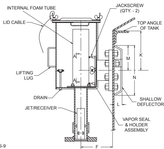
FOAM CHAMBER SECTION WITH SHALLOW DEFLECTOR
