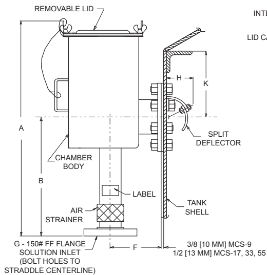
FOAM CHAMBER WITH SPLIT DEFLECTOR
