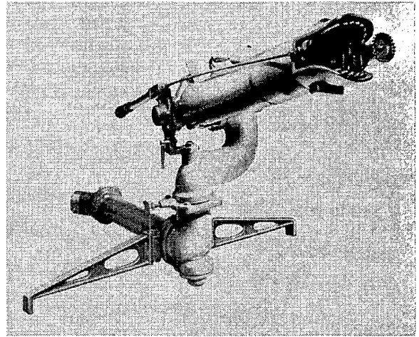
FIGURE A.3.3.18(e) Portable Foam-Water Monitor.
