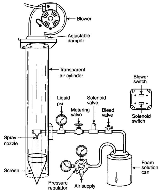
FIGURE H.2(a) High-Expansion Foam Quality Test Generator.
