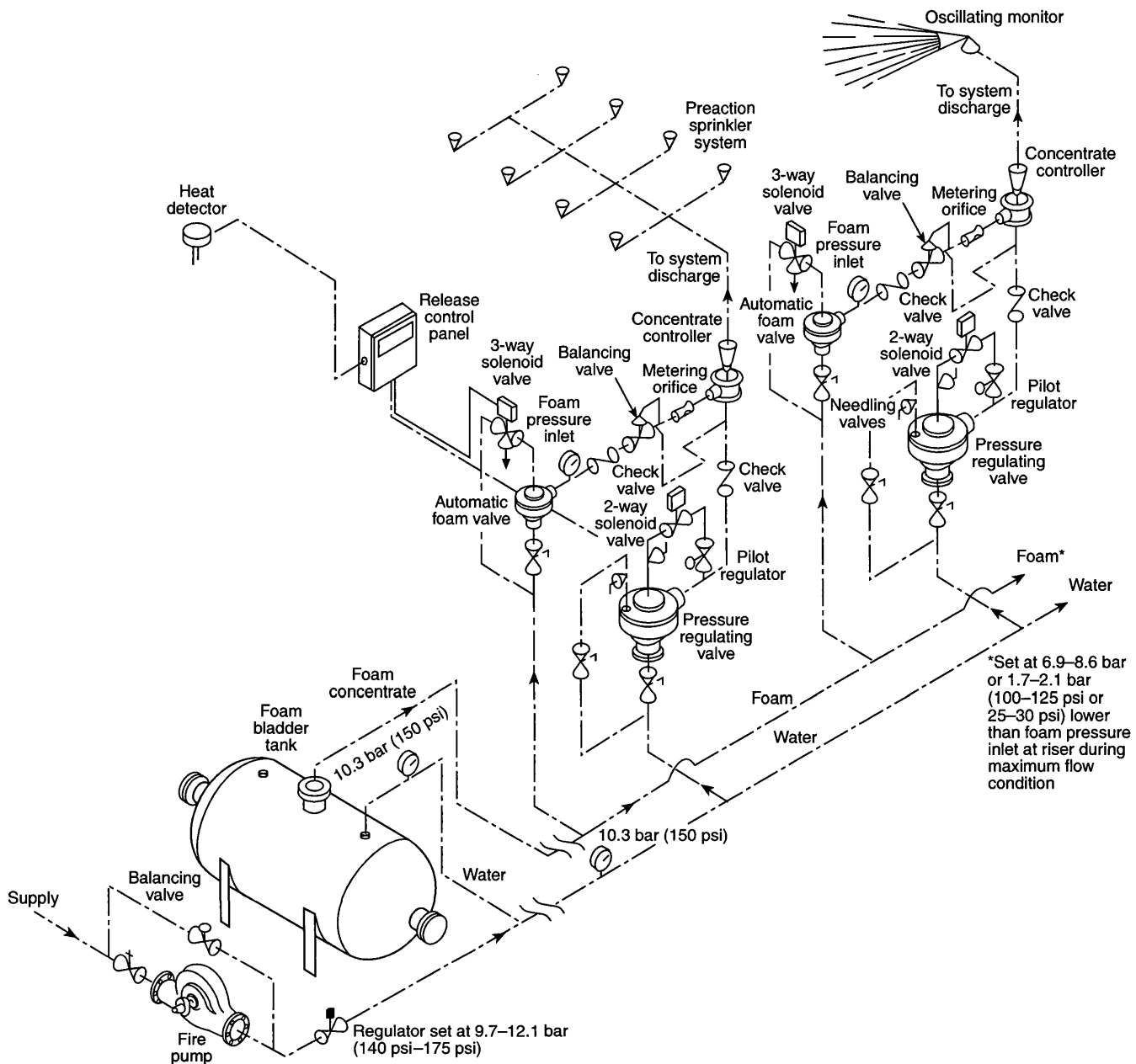
FIGURE A.3.3.25.1.1(b) In-Line Balanced Pressure (Bladder Tank Type) Proportioning with Multiple Injection Points.
