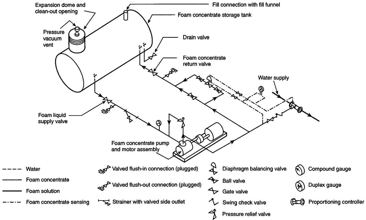
FIGURE A.3.3.25.1 Balanced Pressure Proportioning (Pump-Type) with Single Injection Point.
