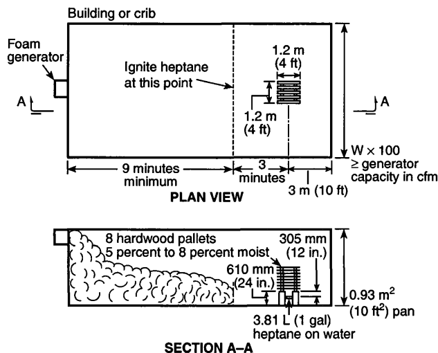
FIGURE H.1 Fire Performance Test.
