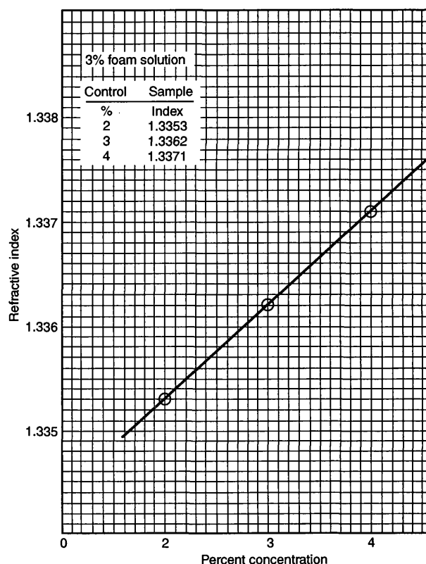
FIGURE D.2.1.1.2 Typical Graph of Refractive Index Versus Foam Concentration.
