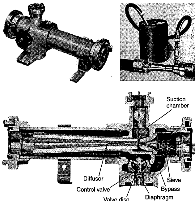
FIGURE A.3.3.6 In-Line Eductor.
