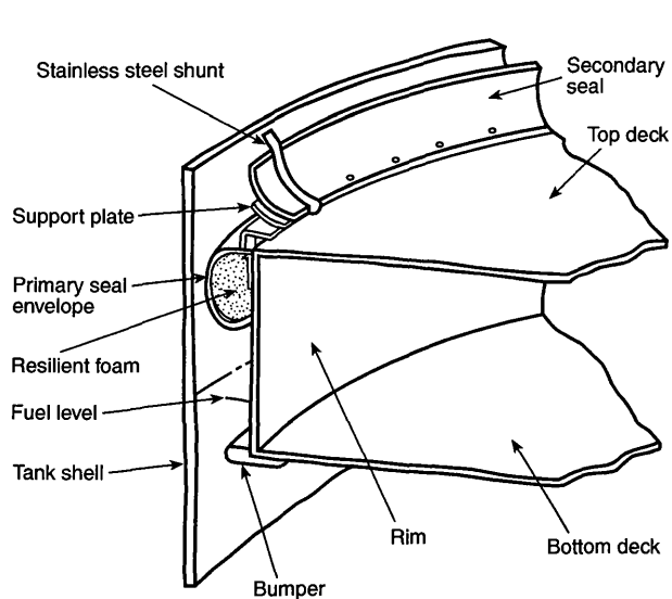
FIGURE 5.3(c) Double Seal System for Floating Roofs.
