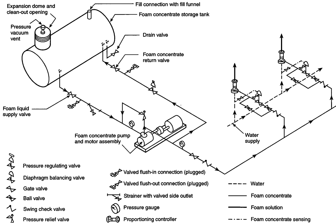
FIGURE A.3.3.25.1(a) In-Line Balanced Pressure (Pump-Type) Proportioning with Multiple Injection Points.
