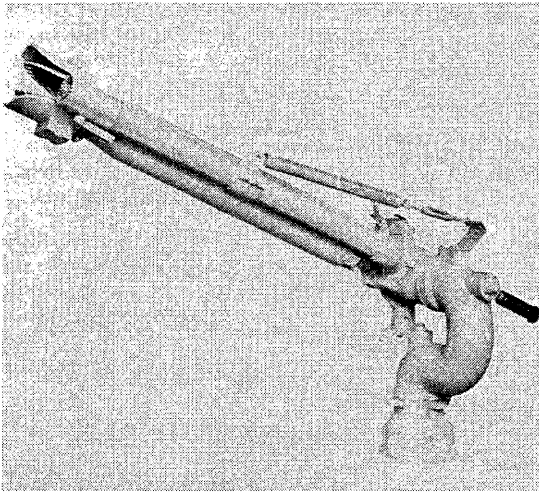
FIGURE A.3.3.18(b) Adjustable Straight Stream-to-Fan Pattern Foam-Water Monitor.
