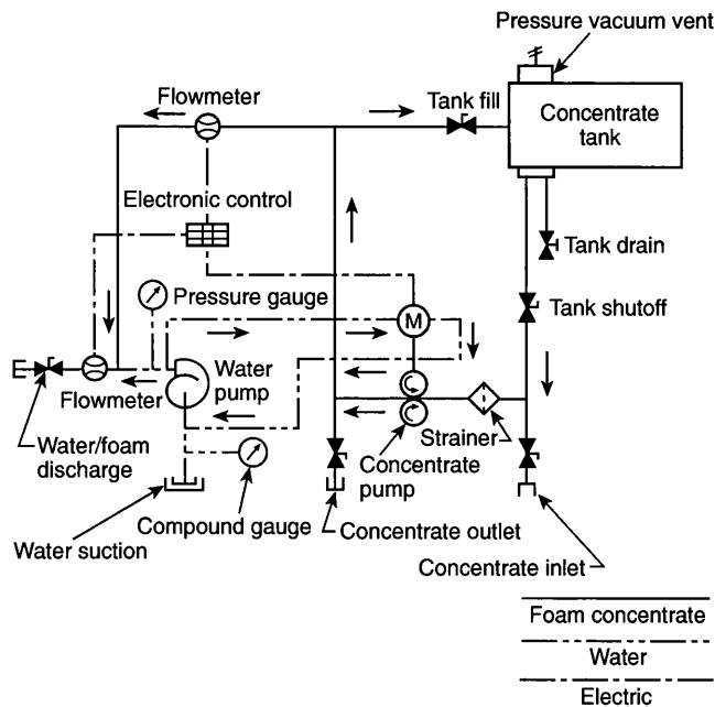
FIGURE A.3.3.25.2(d) Water Turbine-Driven Flow-Sensing Direct Injection Foam Proportioning System.
