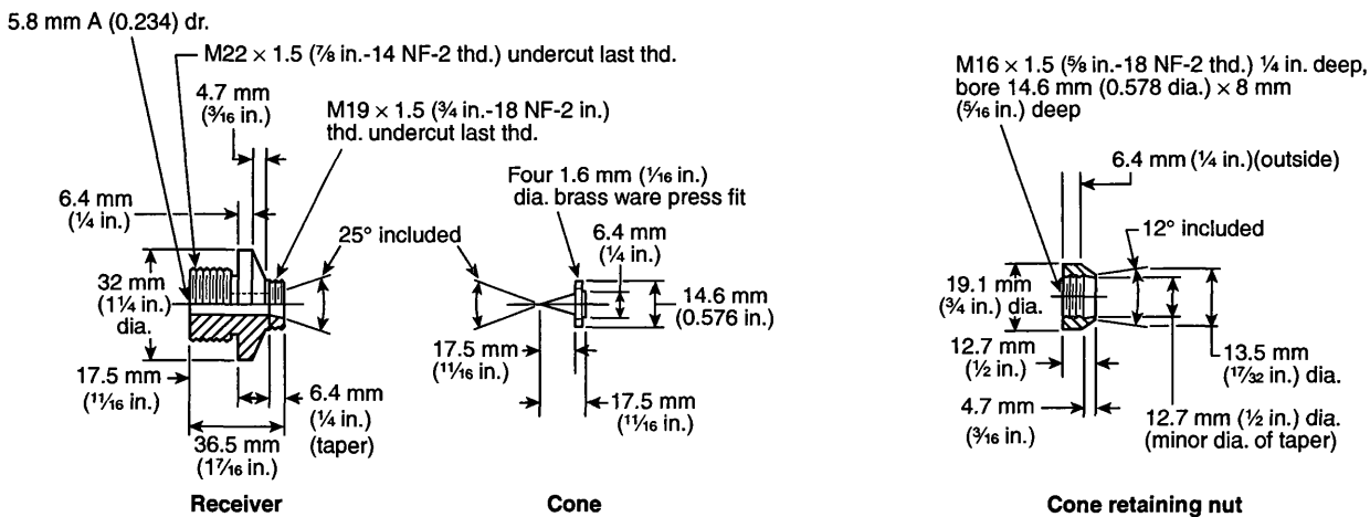
FIGURE G.3.2 Test Nozzle.
