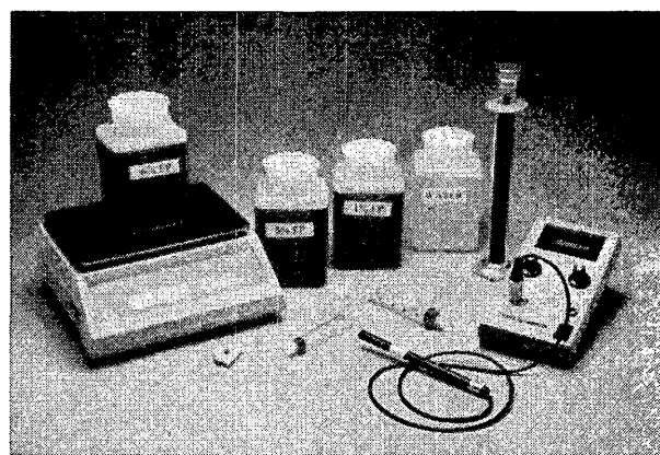
FIGURE D.2.1.2 Equipment Needed for Conductivity Method of Proportioning Measurement.
