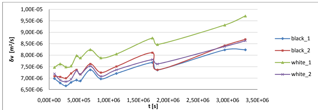
Figure 4.6 Vapor permeability coefficient of Cup method samples.
