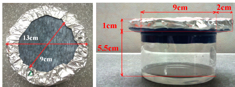
Figure 4.3 Cup method dimensions.
